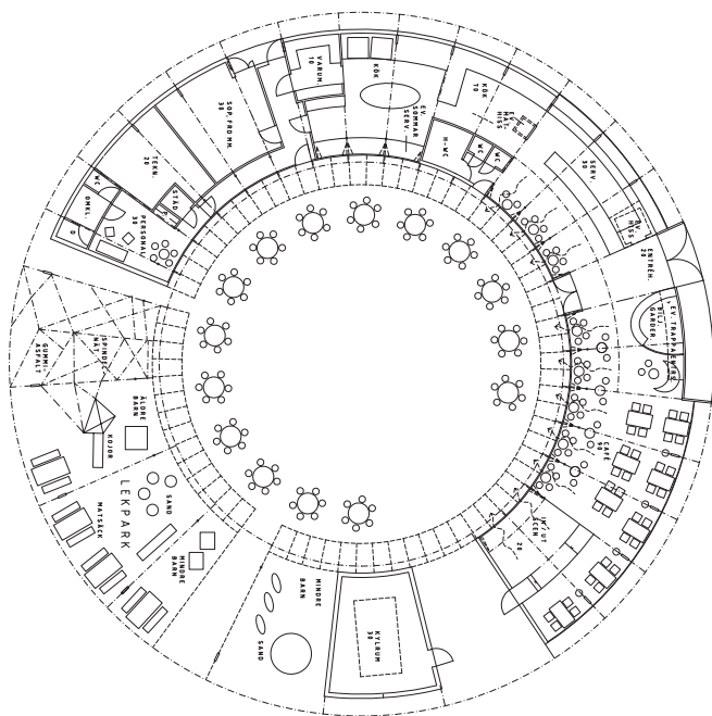
PLAN 1 :400
